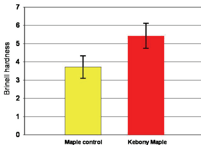
Figure 6: Brinell hardness of unmodified control maple and Kebony Maple
